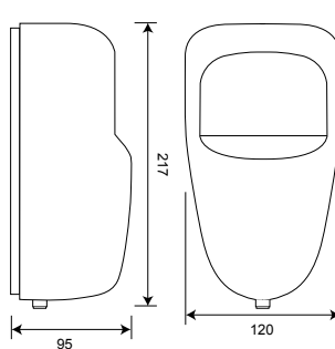
AC00-020 / AC00-019 Virtual Janitor - White / Chrome
