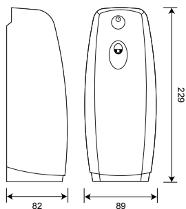
AC00-011 LCD FrAGRANCE dispenser - White
