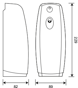
AC00-045 LCD FrAGRANCE dispenser - Chrome
