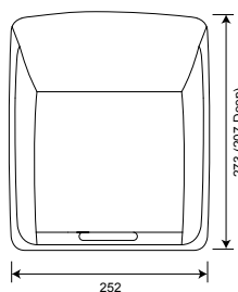
AC00-005 Hand dryer 2100w, white plastic
