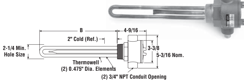
E4TP — Dimensions (Inches)
