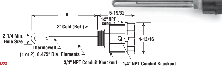
E4TP — Dimensions (Inches)
