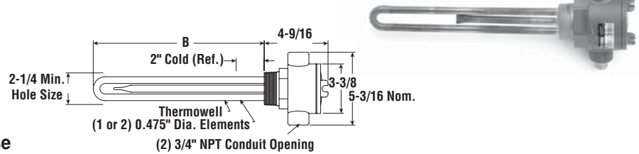
E4TP — Dimensions (Inches)
